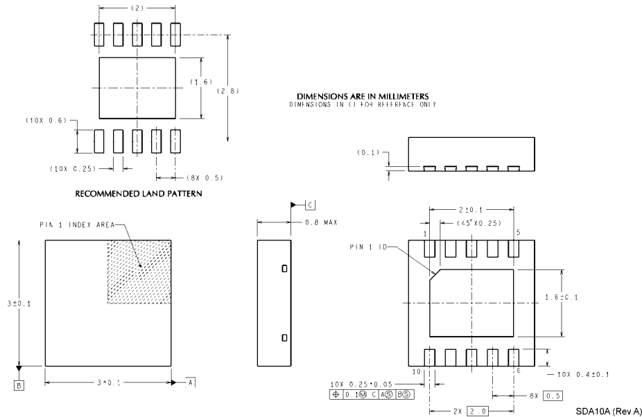
10-Lead LLP Order Numbers DAC102S085C1SD NS Package Number SDA10A
